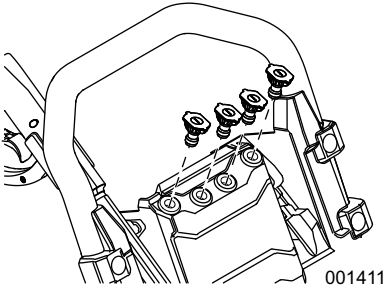
Figure 2-3. Insert Nozzles
